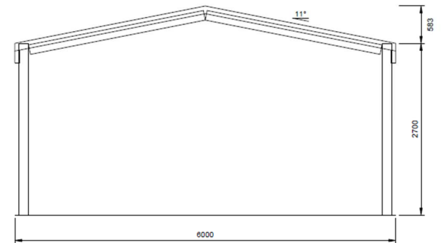
3 REAR ELEVATION
