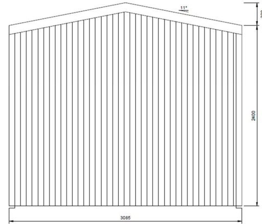
1 REAR ELEVATION 3 SCALE: 1:25 FRAME #2
