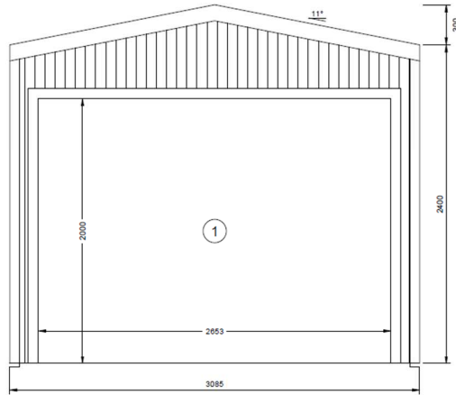
2 FRONT ELEVATION 3 SCALE: 1:25 FRAME #1
